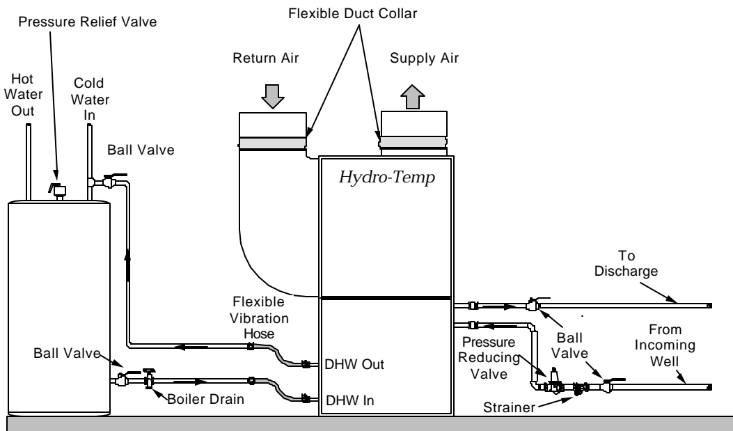
Figure 4.1 Closed Loop Installation with Demand Hot Water
