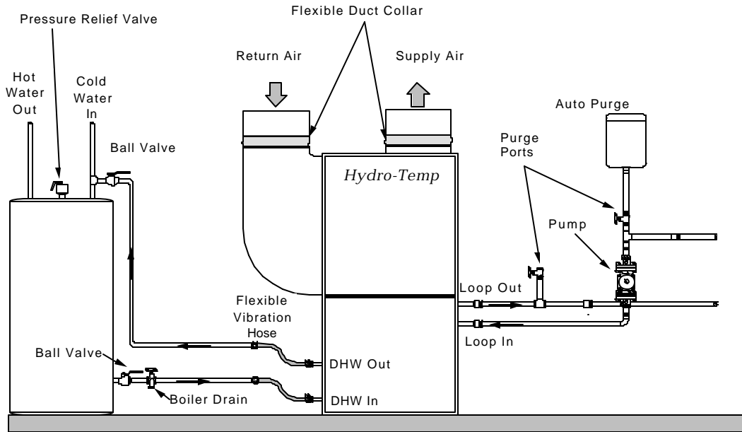
Figure 4.1 Closed Loop Installation with Demand Hot Water
