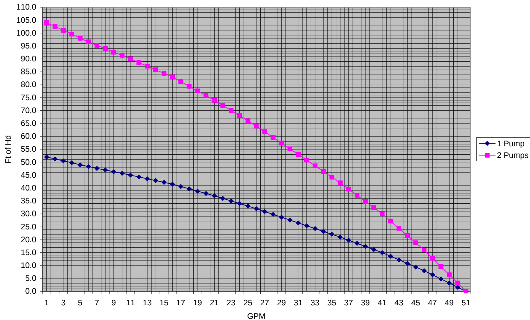
Bell & Gossett PL 55 Pump Curve
