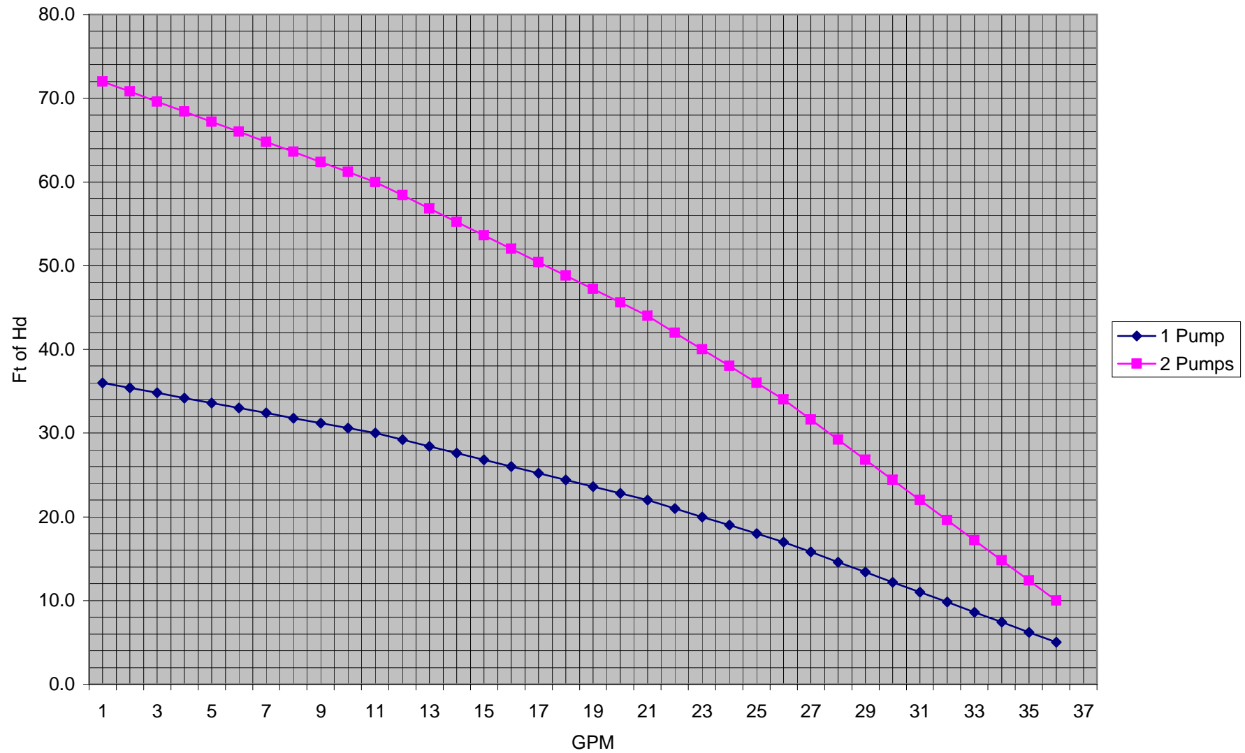
Bell & Gossett PL 36 Pump Curve
